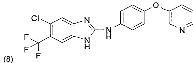
(5-Chlor-6-trifluormethyl-1H-benzimidazol-2-yl)-[4-(pyridin-3-yloxy)-phenyl]-amin
